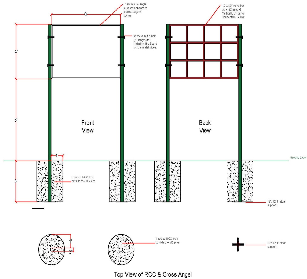
Detail diagram of AVCB Phase-II Signboard
